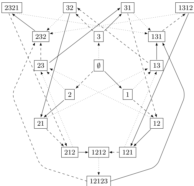
Figure 2: The Canon automaton for W_{(3,3,4)}
