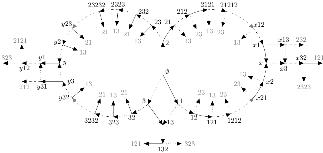
Figure 4: Class II triangle groups; a, b > 4 with a even and b odd. Conventions as in Figure 3
