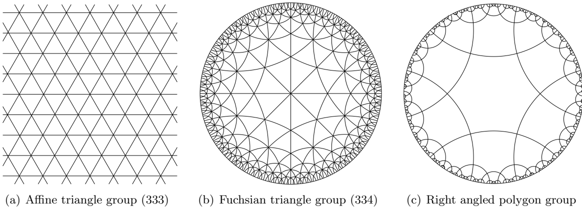
Figure 1: Triangle and polygon groups
