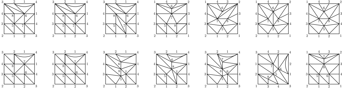
Figure 4.4: A classification of minimal saw-blade complexes with two blades.
