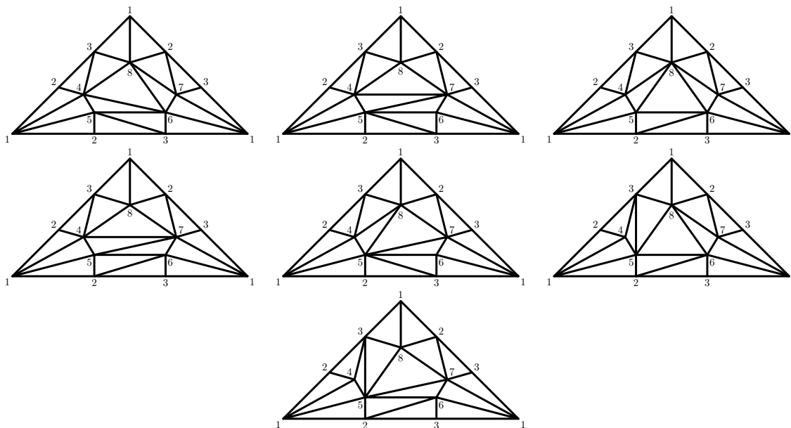
Figure 4.1: A classification of minimal triangulations of the Dunce hat.
